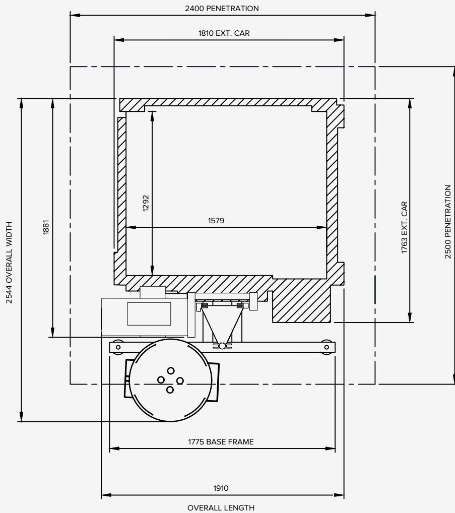
PLAN VIEW
