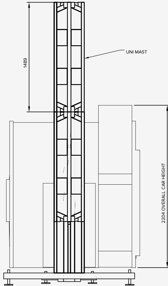
ELEVATION VIEW
